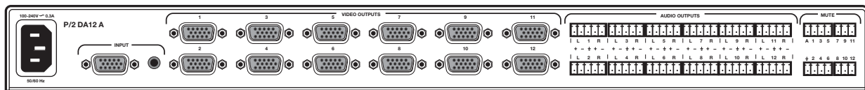
P/2 DA12 A - Back
